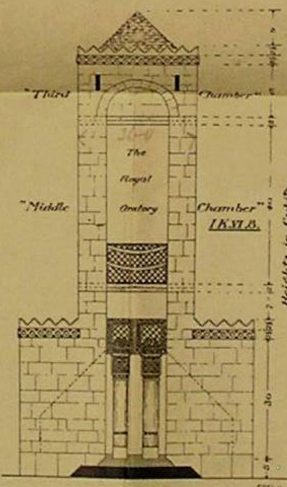
FRONT ELEVATION OF TEMPLE.
